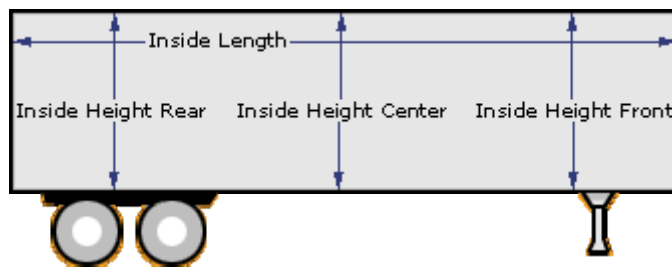
45 ft. or 48 ft. Wedge Trailer
